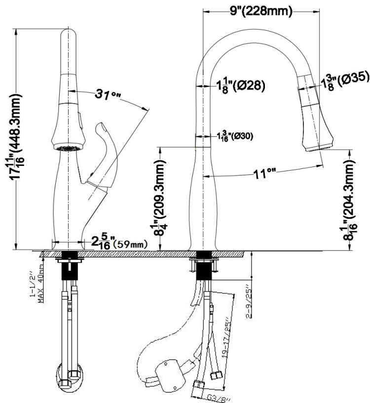
CRITICAL DIMENSIONS
